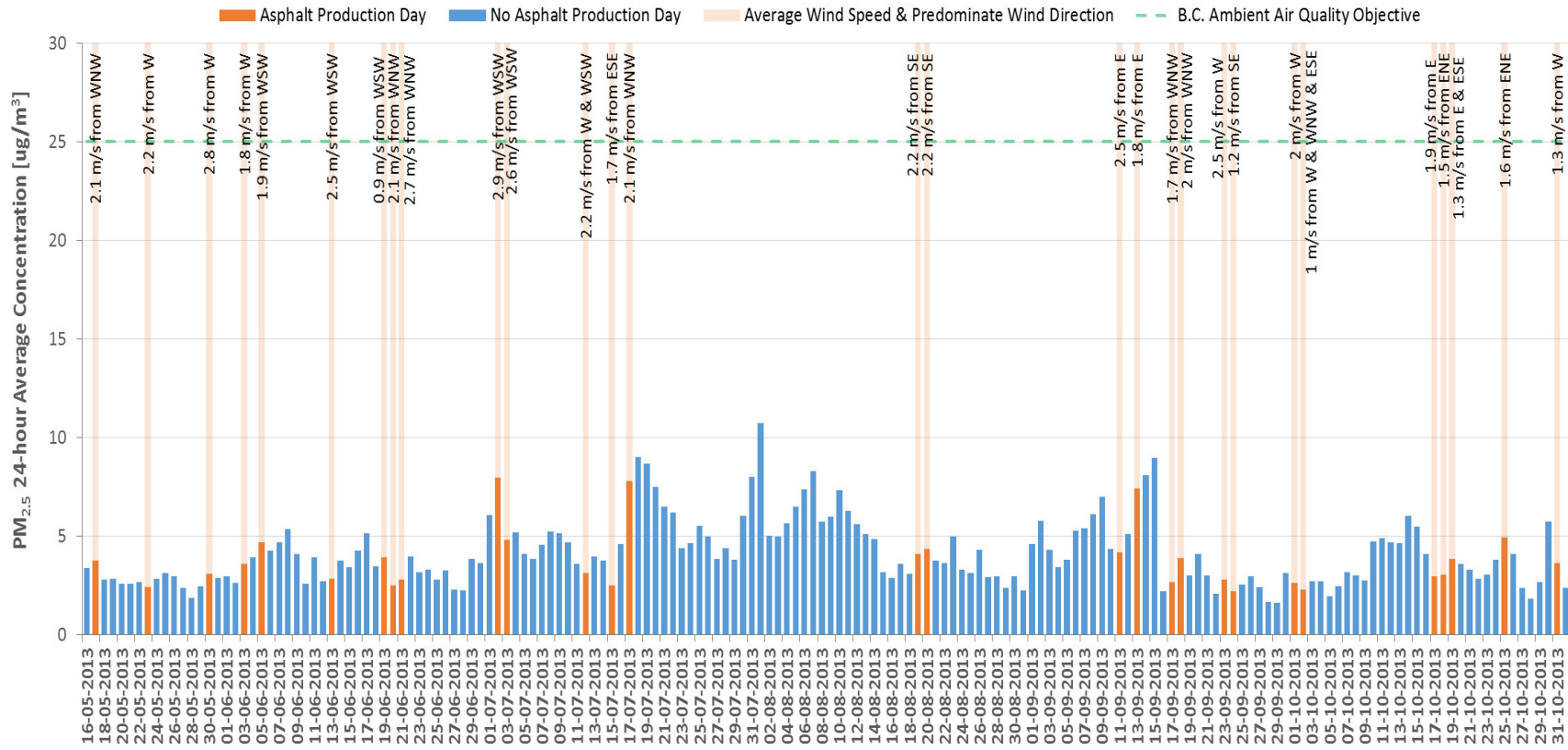
Figure 5-2 Timeseries of Daily Average PM 2.5 Concentrations Monitored at Cheakamus Crossing, 2013
