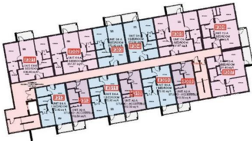
3 Level 2 Floor Plan SCALE 1/8\"/>
