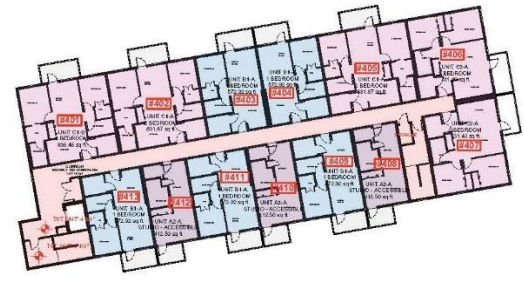
4 Level 3 Floor Plan SCALE 1/8\"/>
