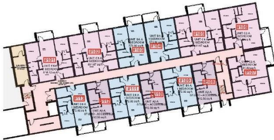
1 Level P1 Floor Plan SCALE 1/8\"/>
