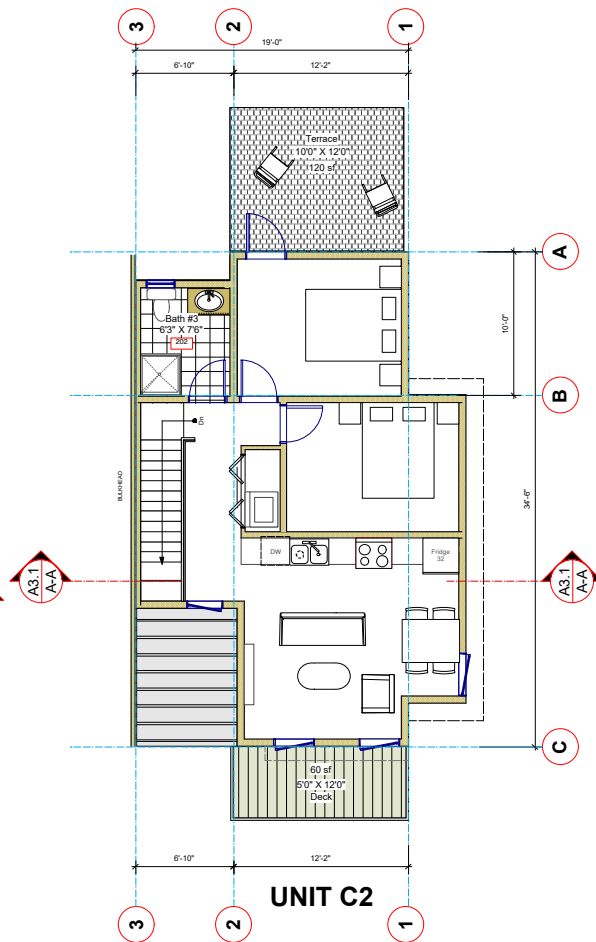
Unit C - Main Floor
