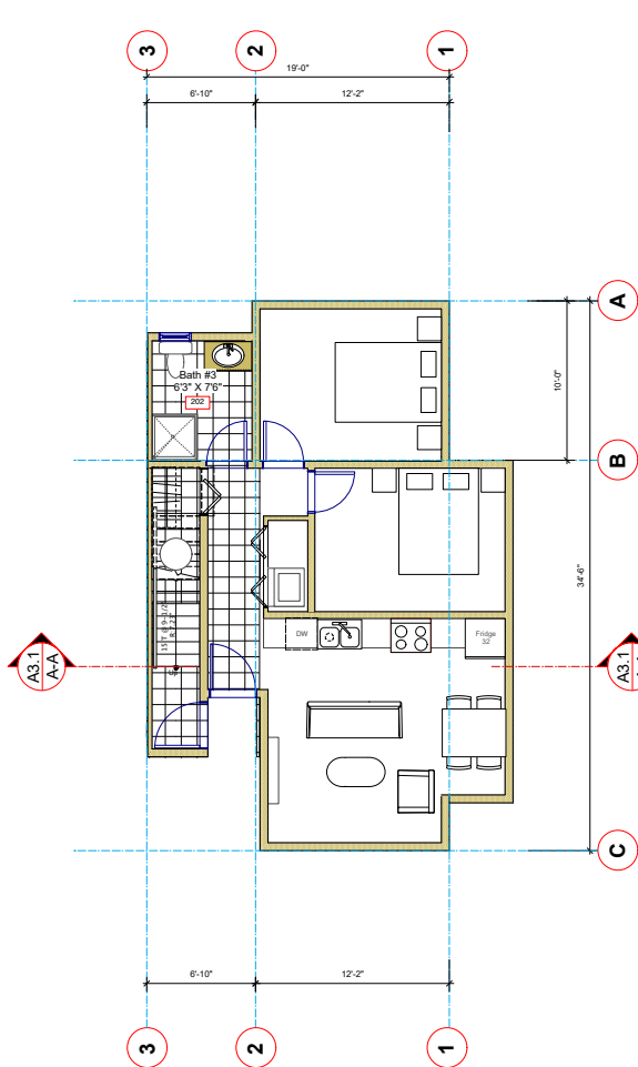
Unit C - Lower Floor
